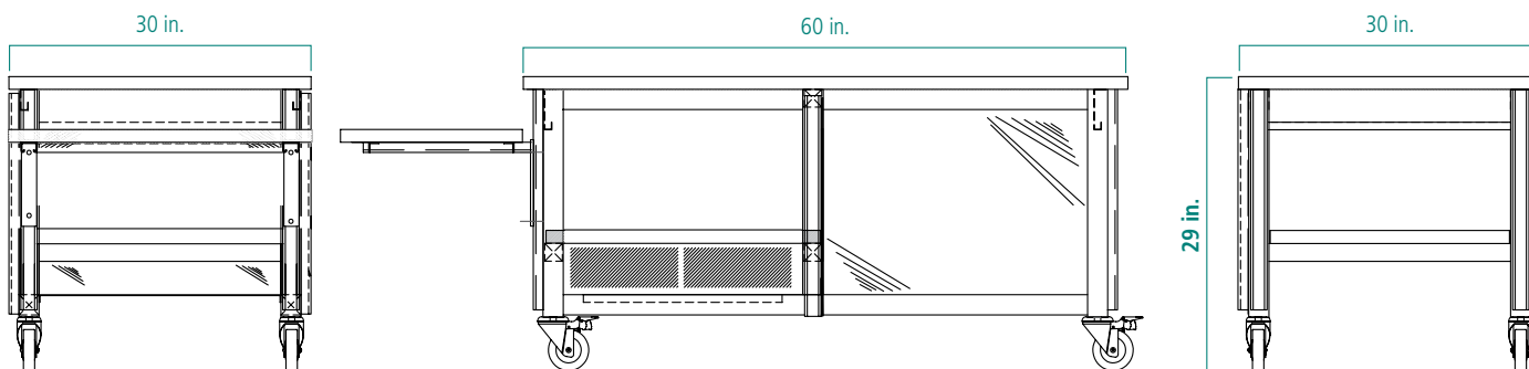
NexION 350 Bench Part No. N8141230 shown as depth/width/height
